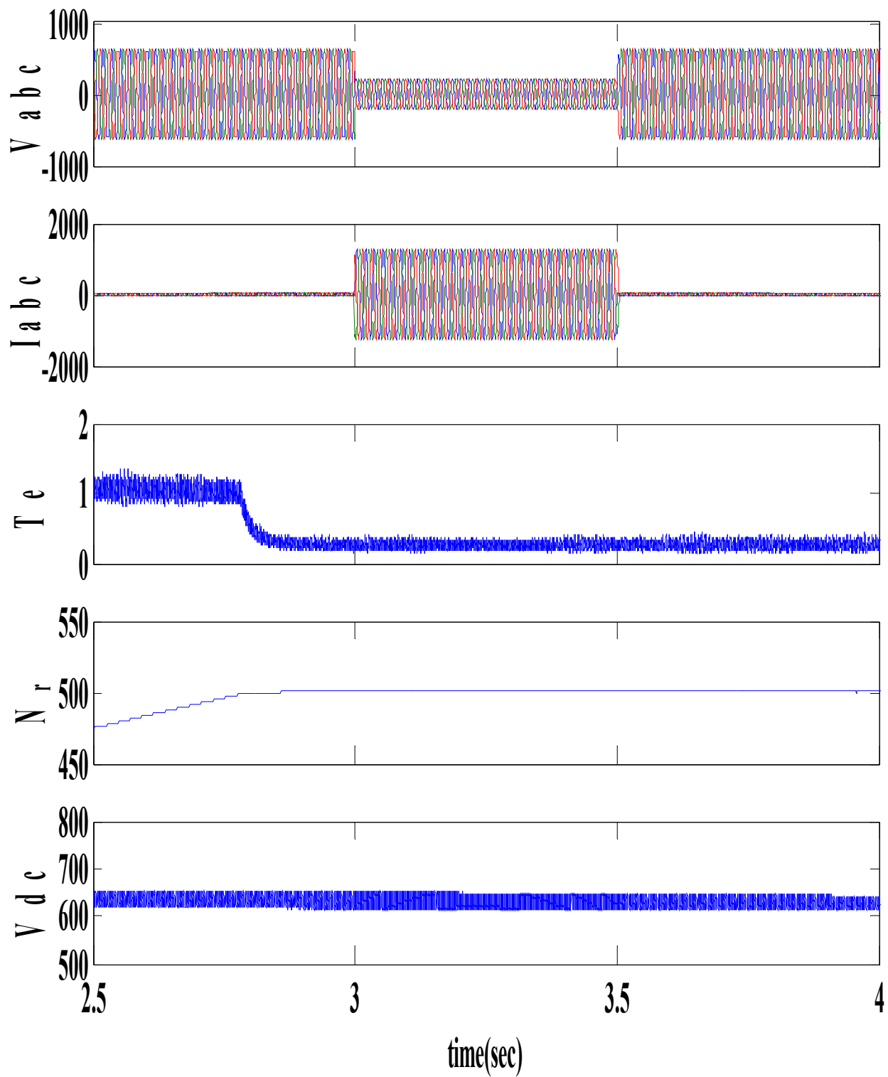
Fig. 5. Performance of ASD's during three-phase symmetrical fault
