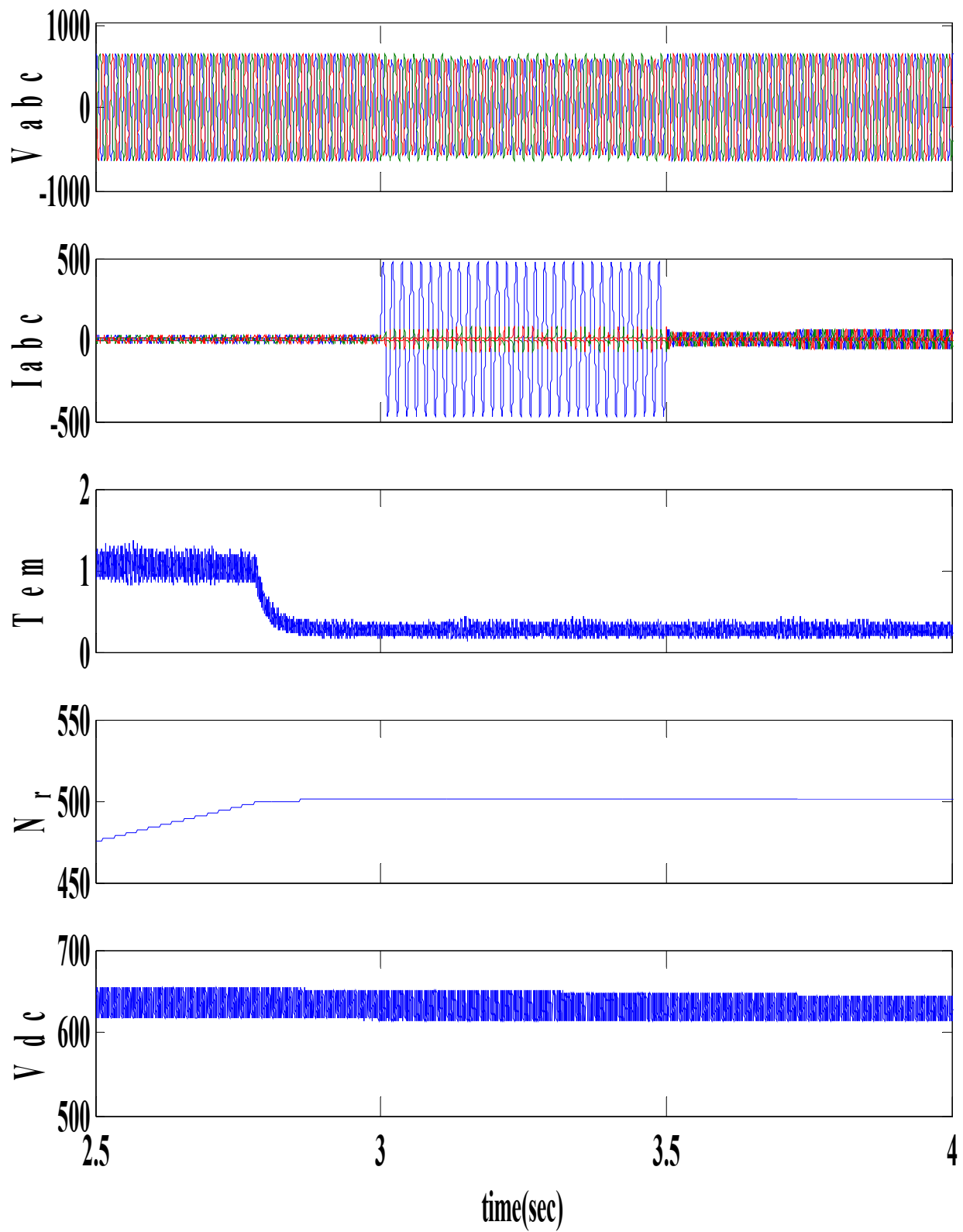
Fig. 6. Performance of ASD's during single-phase line -ground fault
