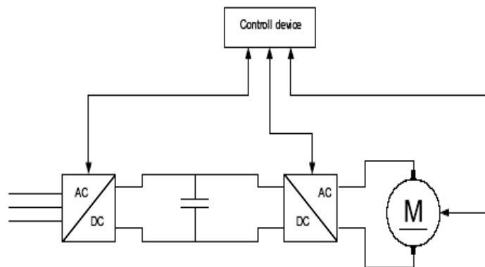
Fig. 1. AC ASD'S topology
