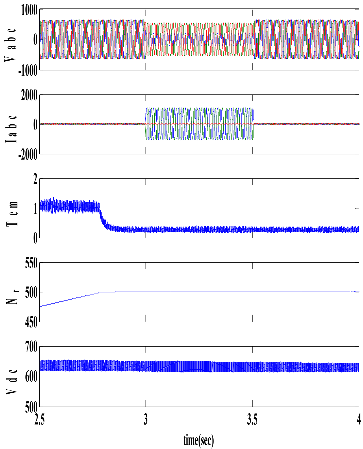
Fig. 7. Performance of ASD's during double line -ground fault
