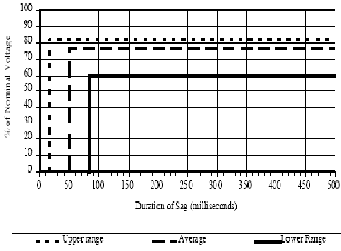
Fig. 3 Voltage tolerance curve of an ASD's (IEEE Std.1346)
